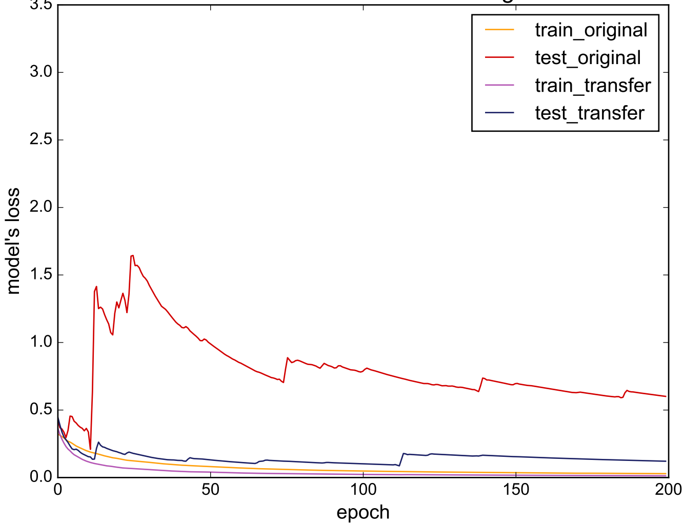
Source: ChlorineConcentration - Target: wafer
