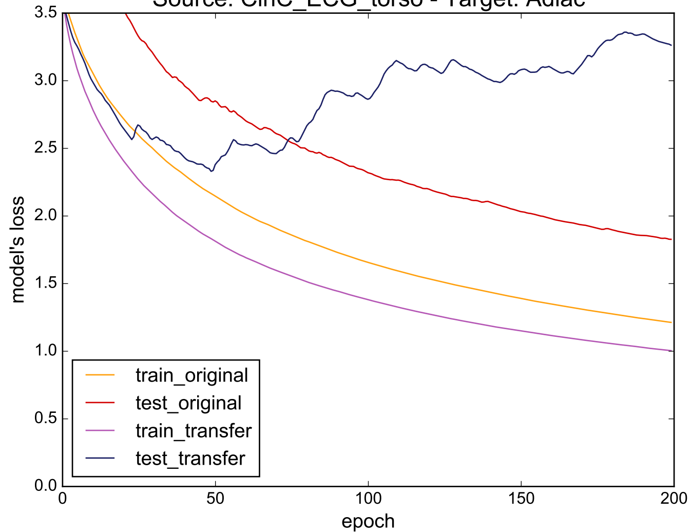
Source: CinC_ECG_torso - Target: Adiac
