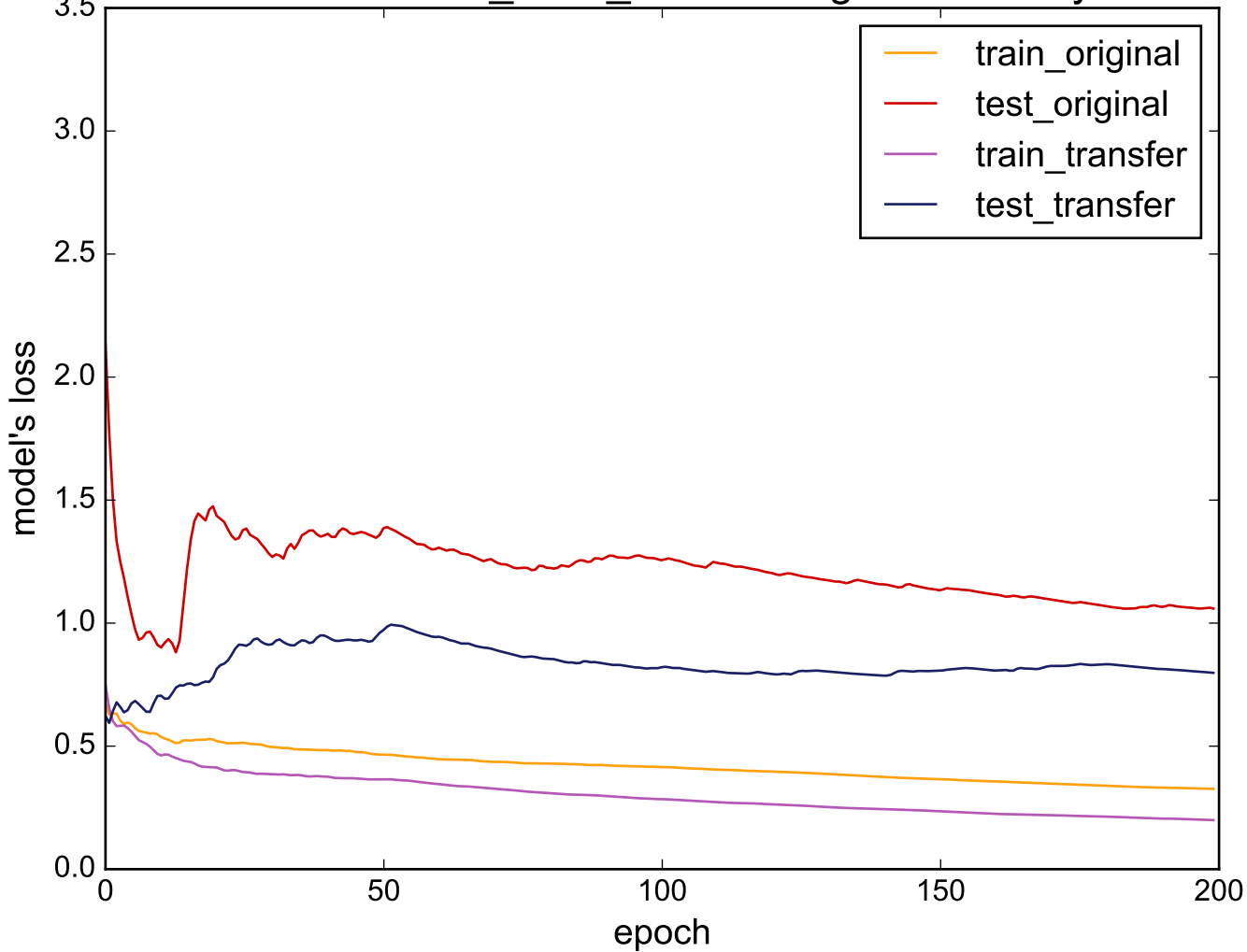
Source: CinC_ECG_torso - Target: BeetleFly
