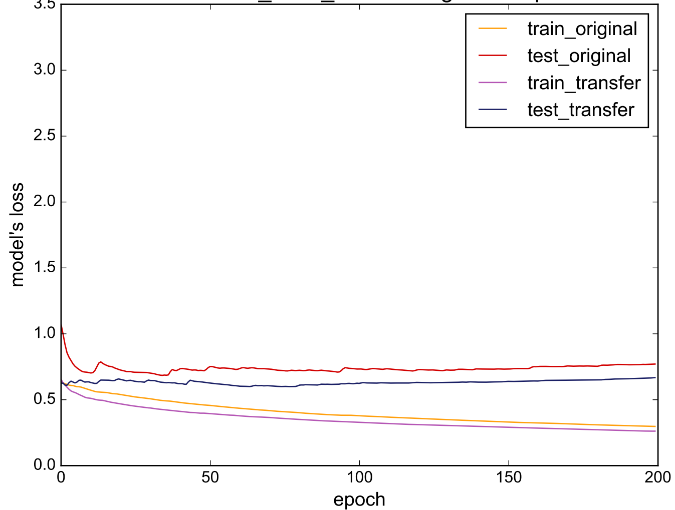
Source: CinC_ECG_torso - Target: Computers
