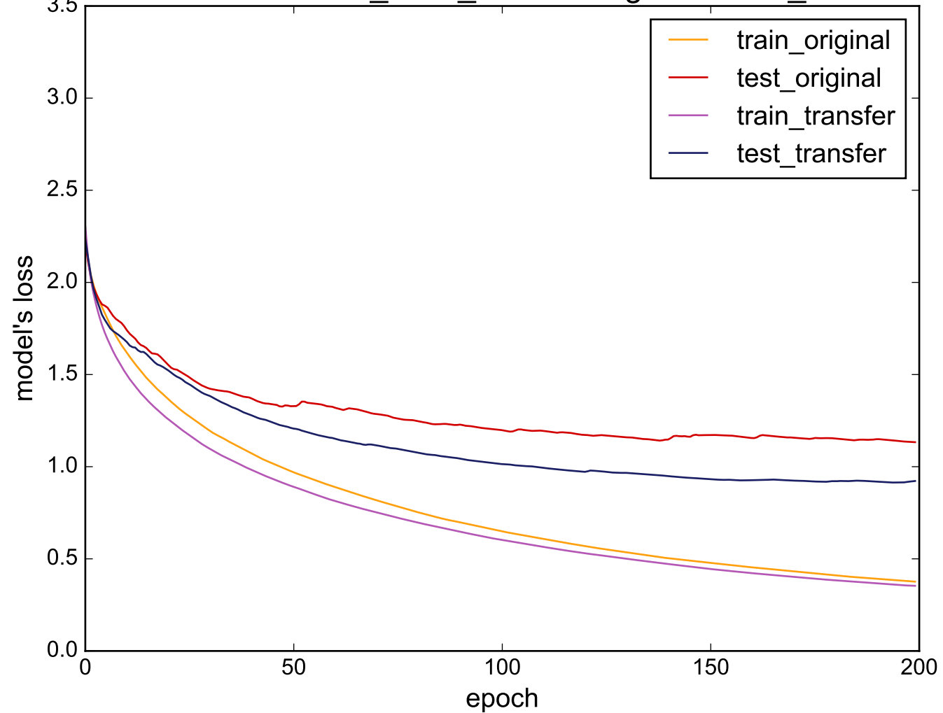
Source: CinC_ECG_torso - Target: Cricket_Y
