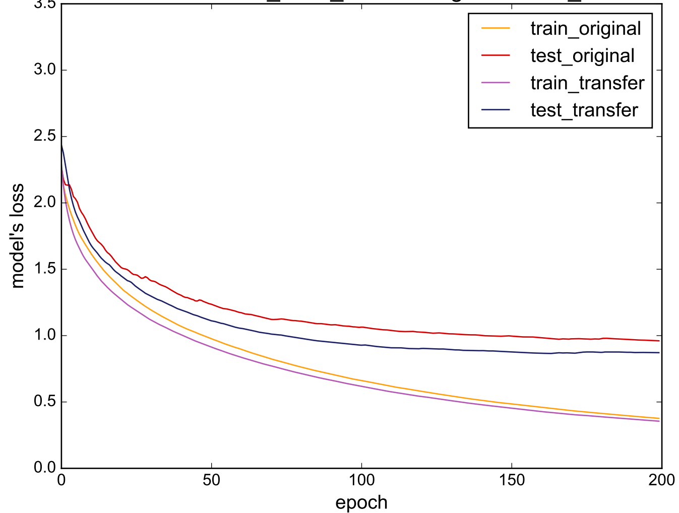
Source: CinC_ECG_torso - Target: Cricket_Z
