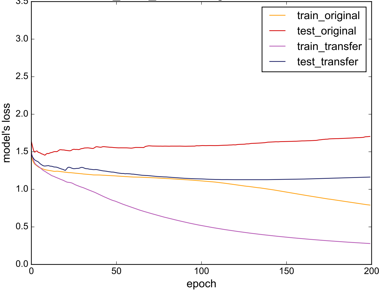
Source: CinC_ECG_torso - Target: DiatomSizeReduction
