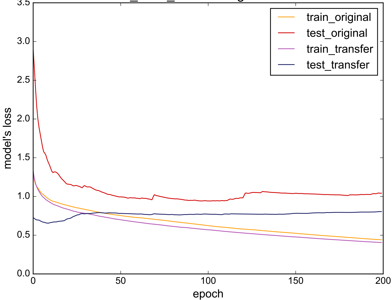
Source: CinC_ECG_torso - Target: DistalPhalanxTW
