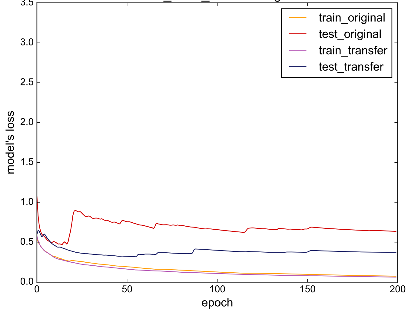
Source: CinC_ECG_torso - Target: ECG200
