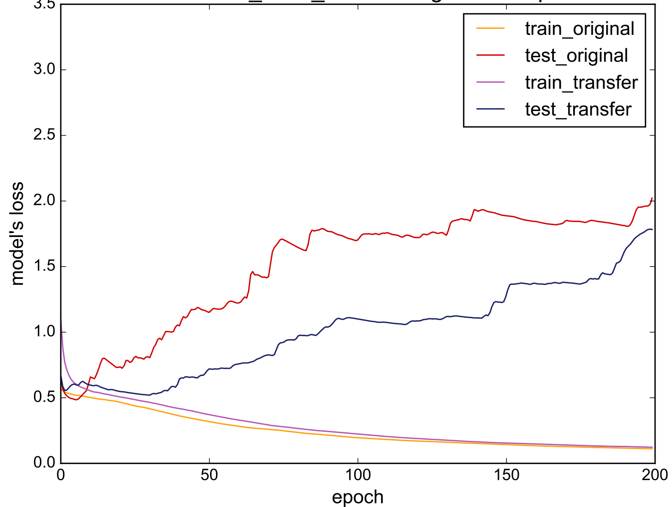
Source: CinC_ECG_torso - Target: Earthquakes
