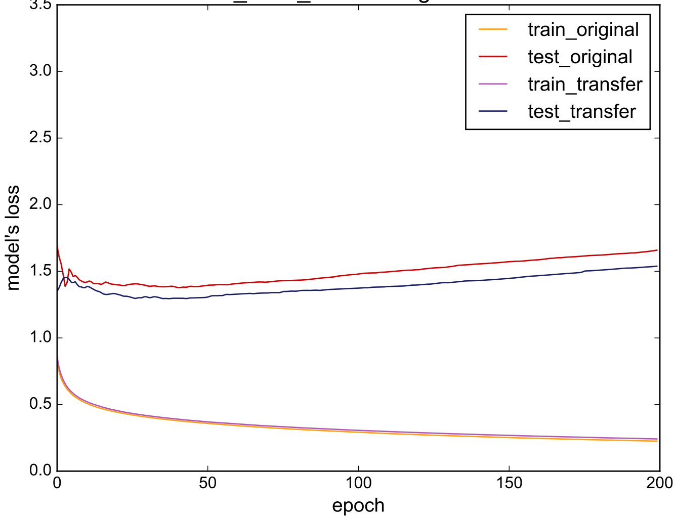
Source: CinC_ECG_torso - Target: ElectricDevices
