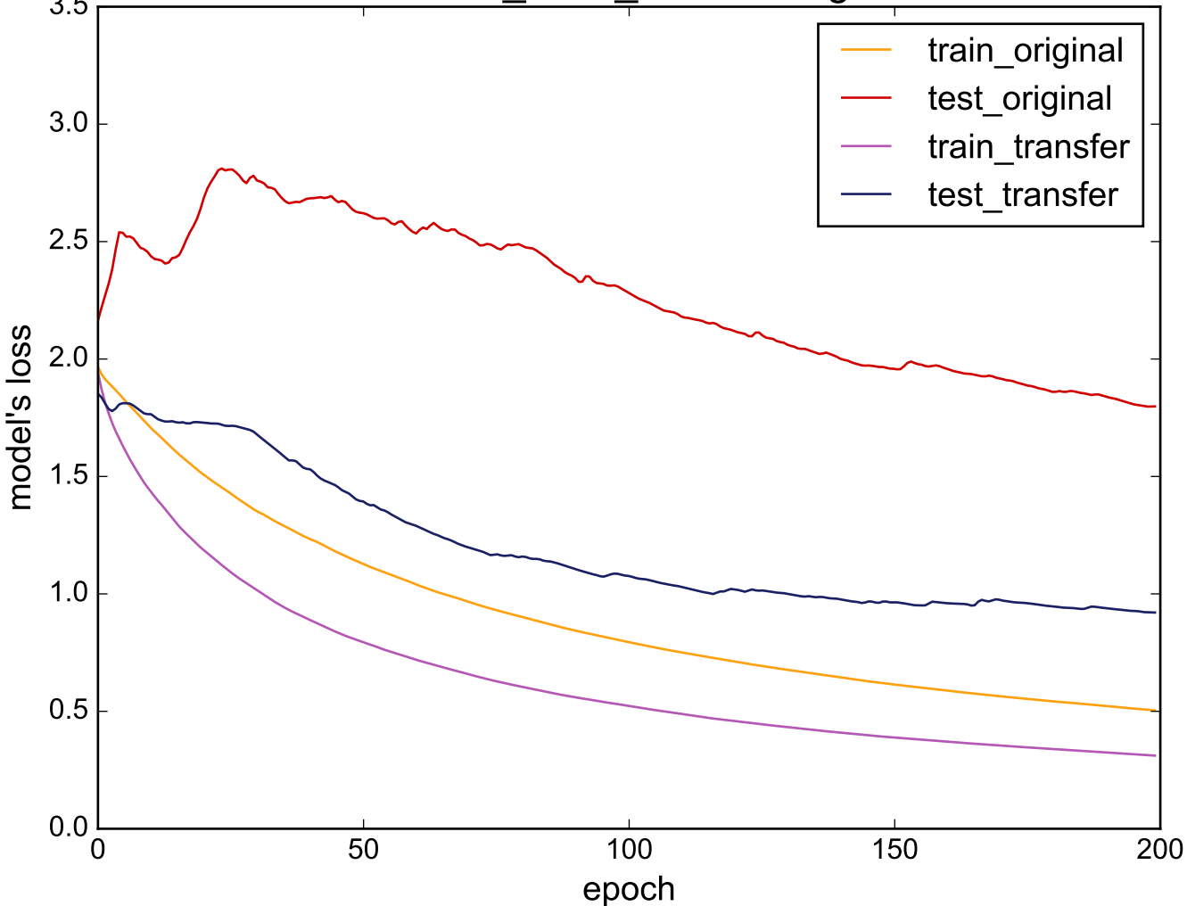
Source: CinC_ECG_torso - Target: FISH
