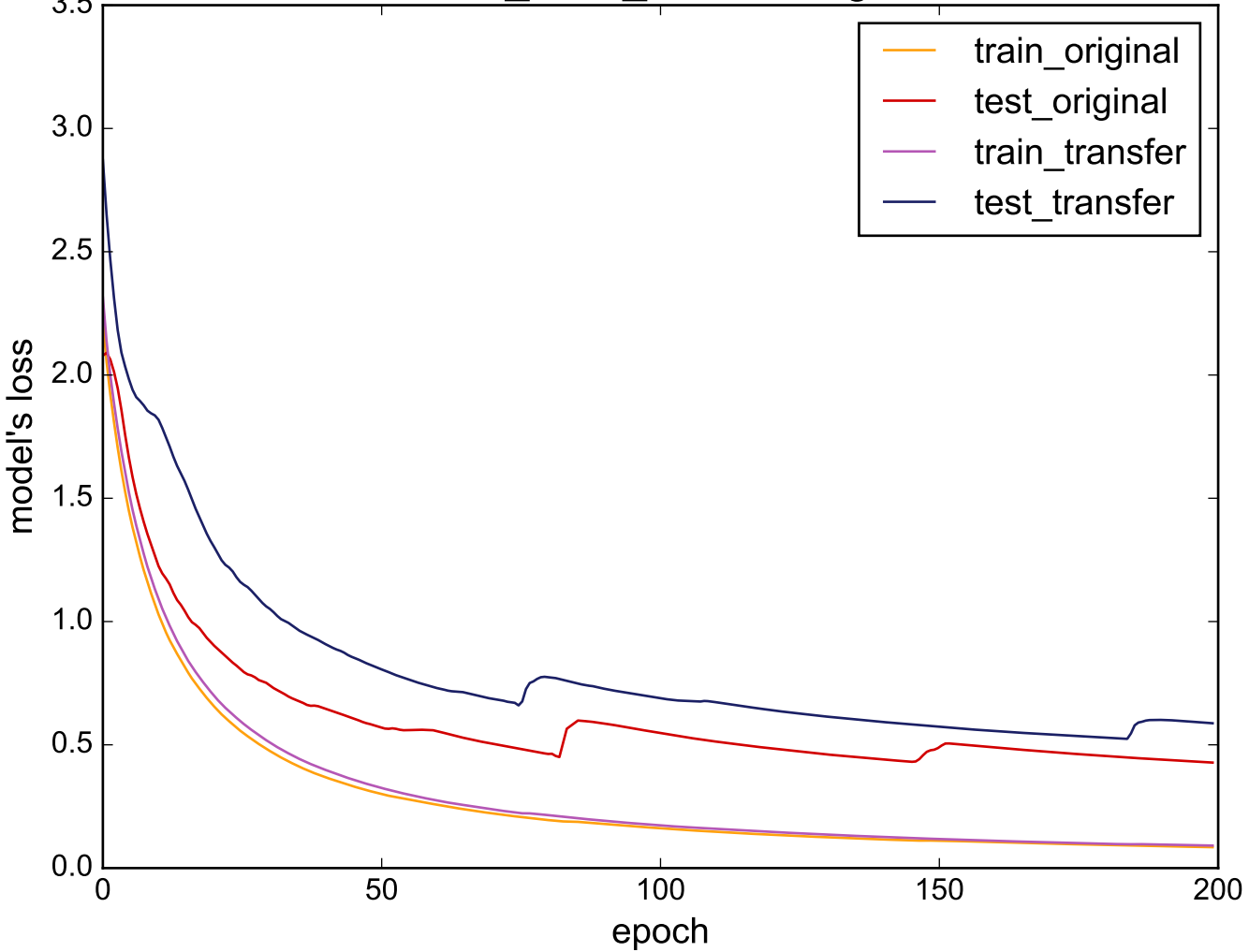
Source: CinC_ECG_torso - Target: FaceAll
