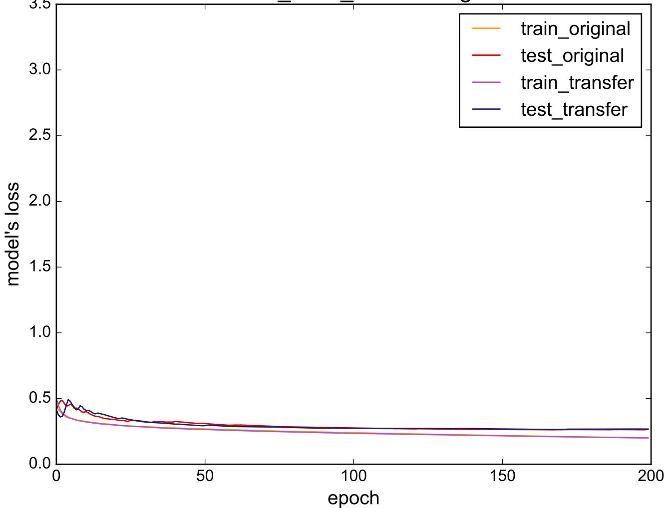
Source: CinC_ECG_torso - Target: FordA
