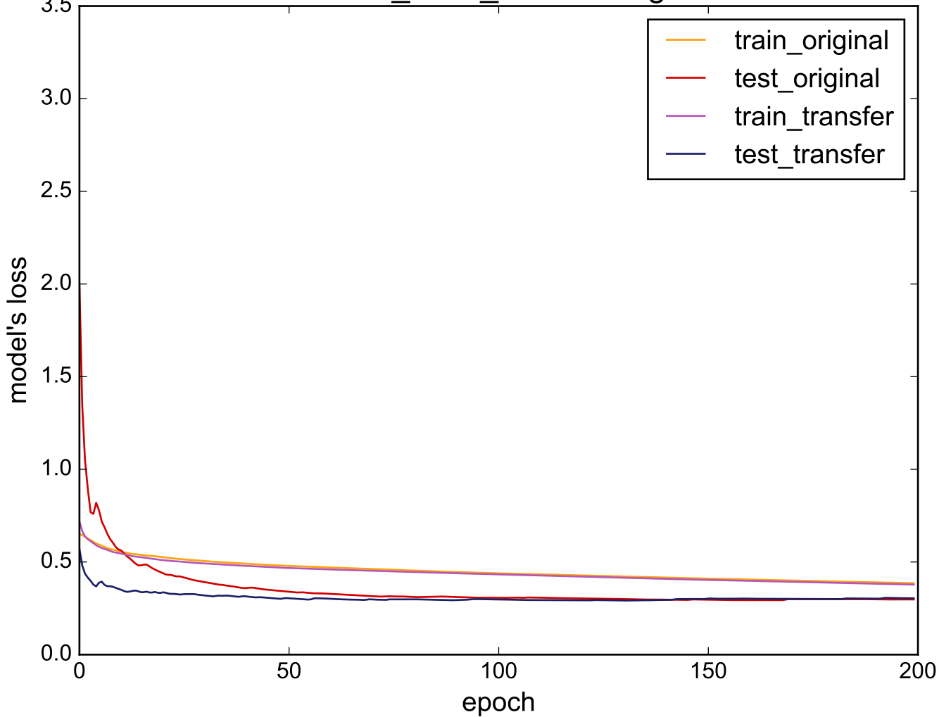
Source: CinC_ECG_torso - Target: FordB
