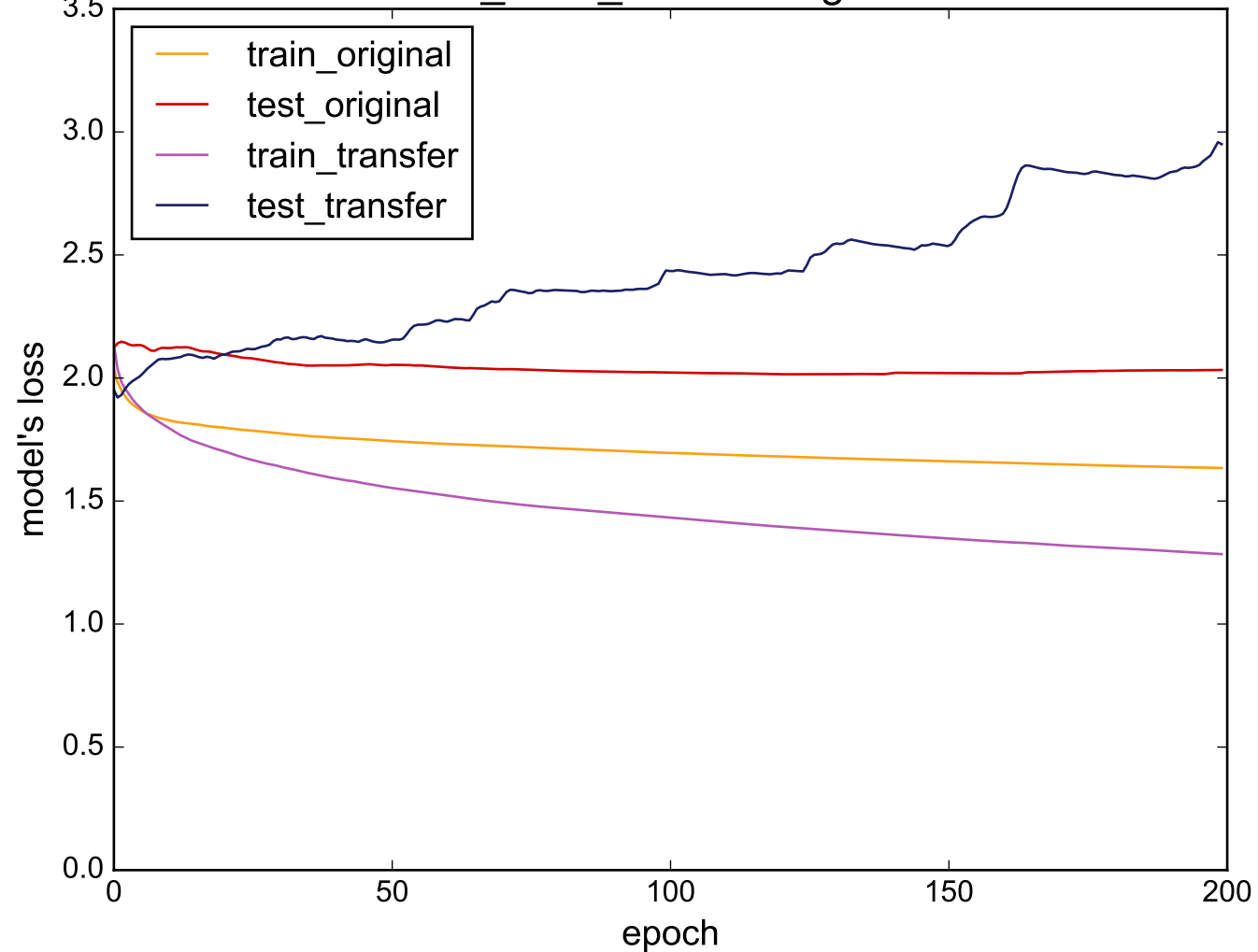
Source: CinC_ECG_torso - Target: InlineSkate
