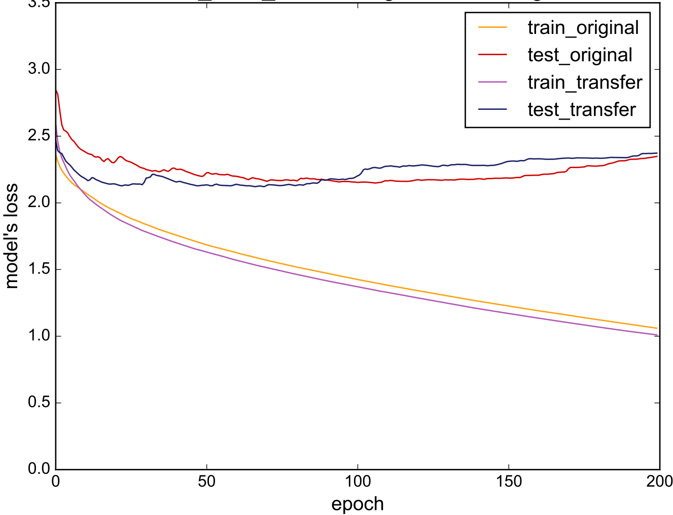
Source: CinC_ECG_torso - Target: InsectWingbeatSound
