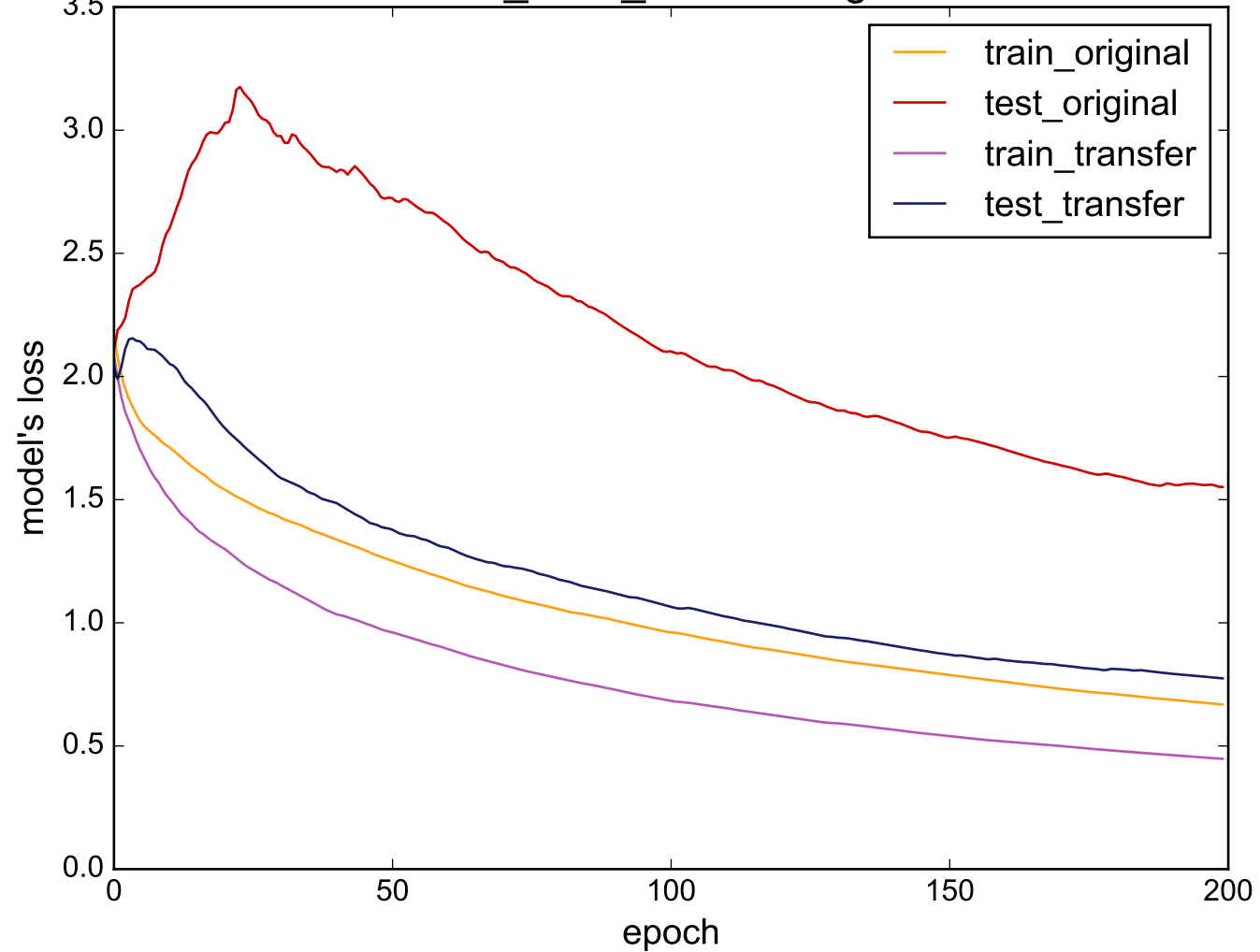
Source: CinC_ECG_torso - Target: MALLAT
