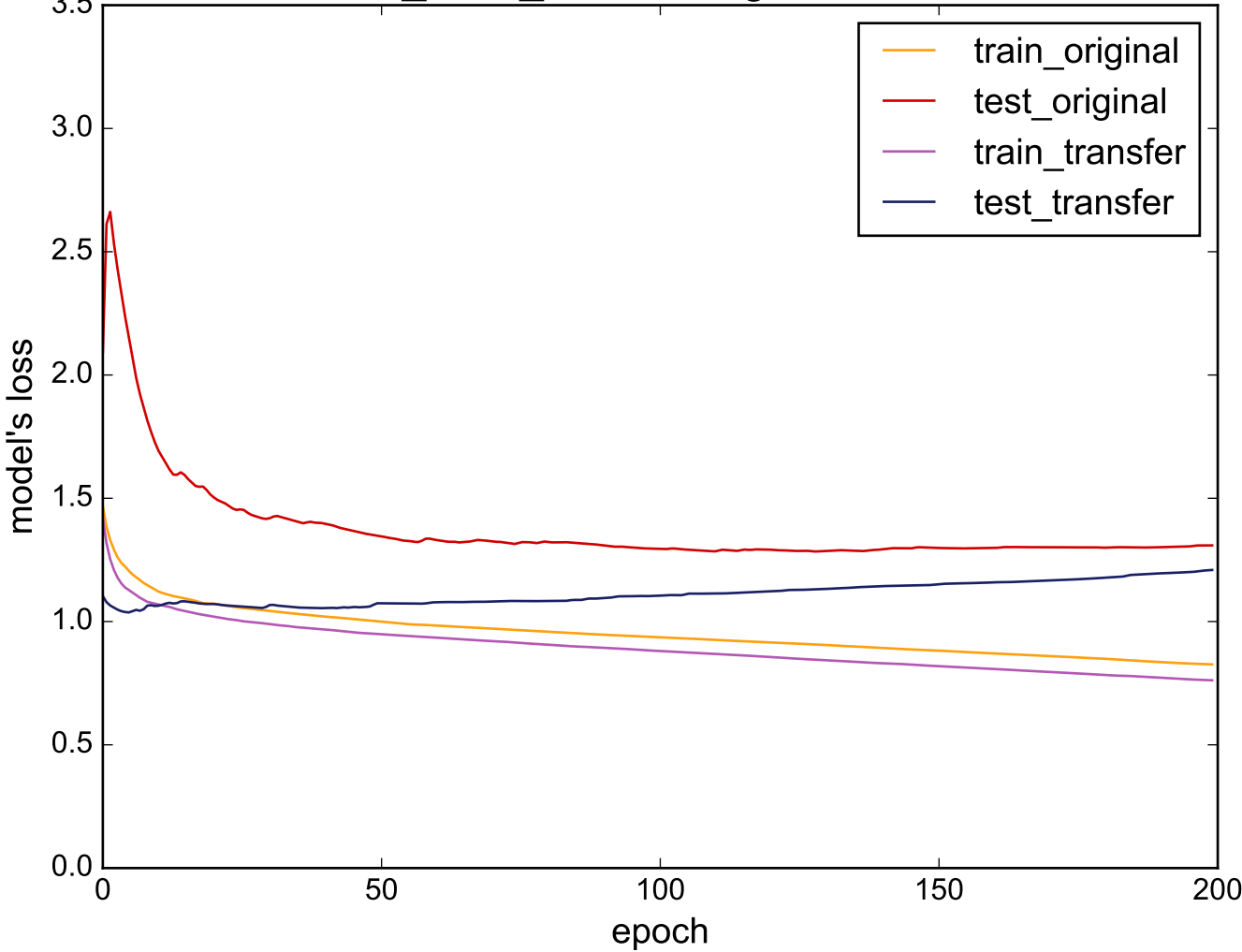
Source: CinC_ECG_torso - Target: MiddlePhalanxTW
