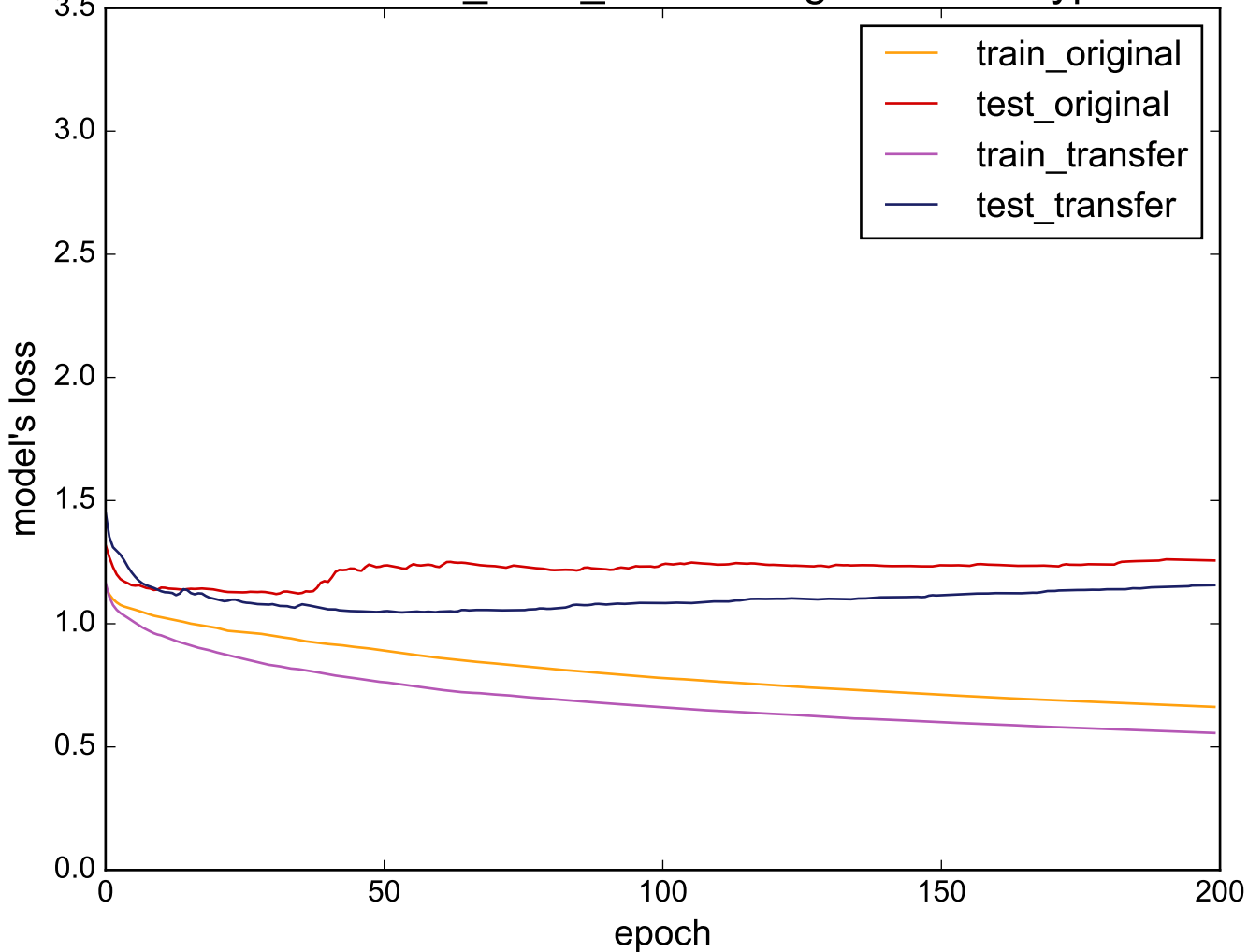
Source: CinC_ECG_torso - Target: ScreenType
