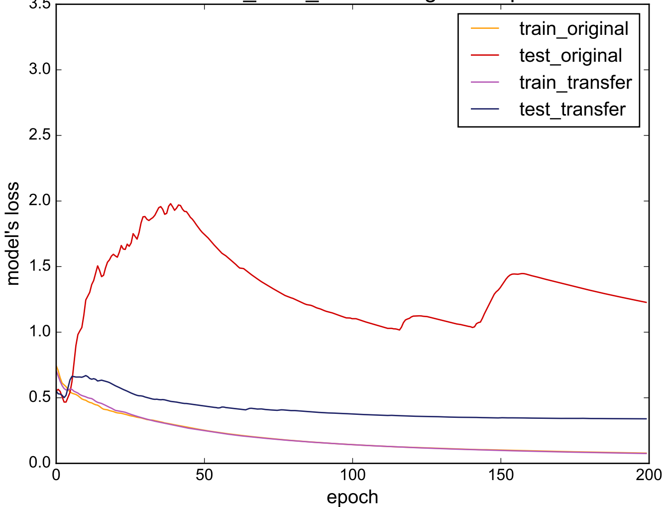
Source: CinC_ECG_torso - Target: ShapeletSim
