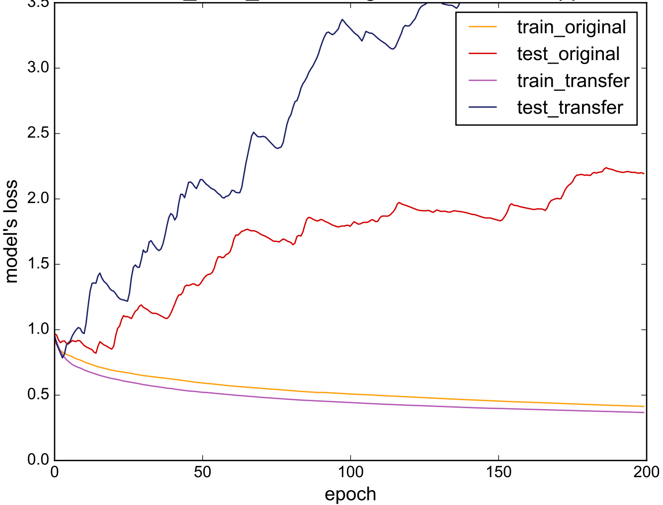
Source: CinC_ECG_torso - Target: SmallKitchenAppliances
