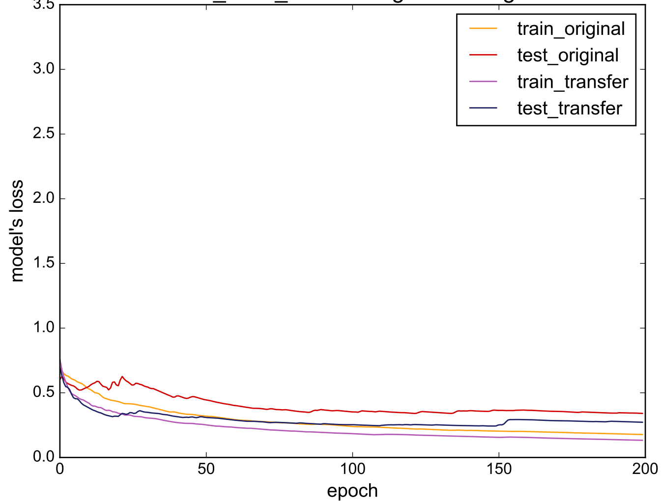
Source: CinC_ECG_torso - Target: ToeSegmentation1
