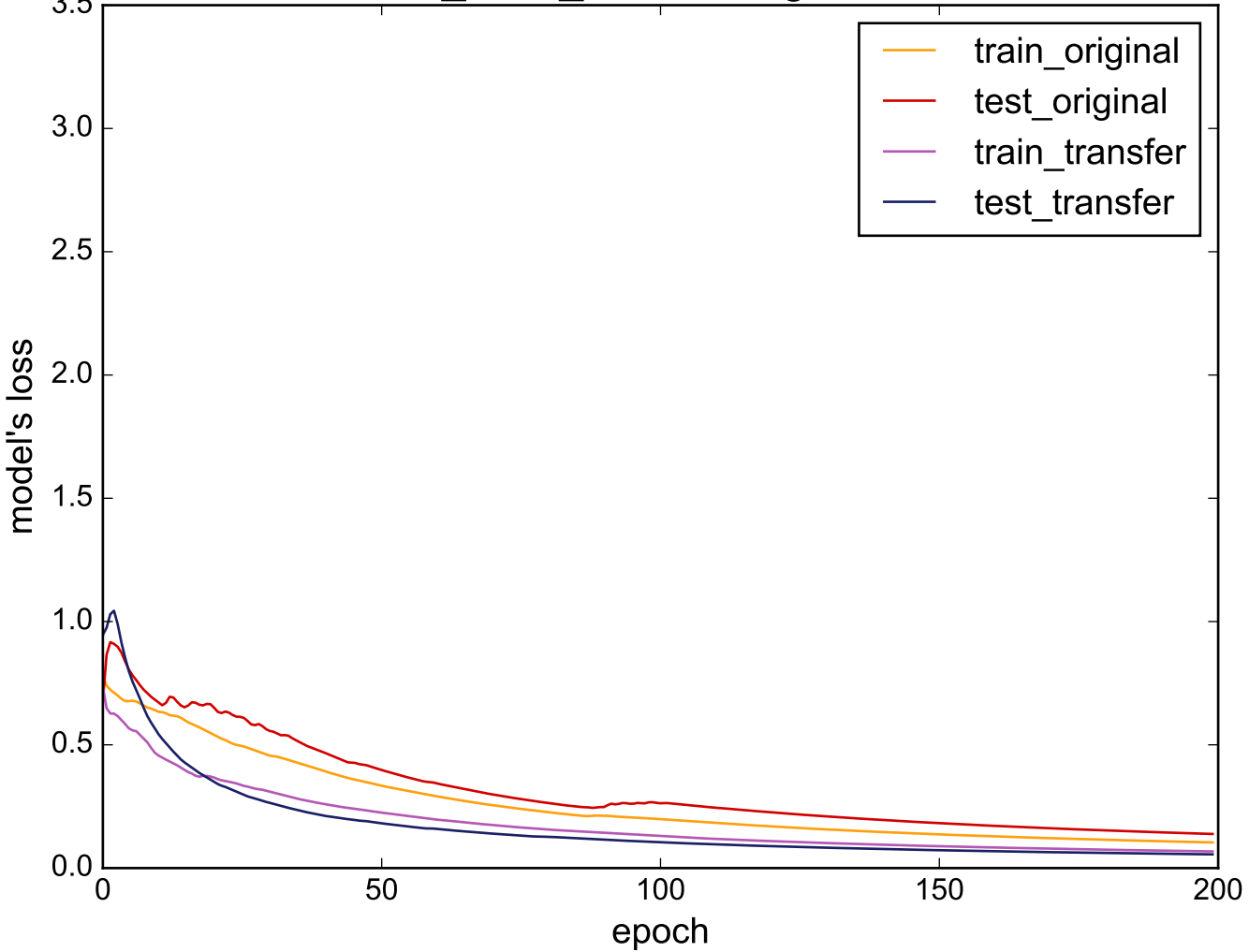
Source: CinC_ECG_torso - Target: TwoLeadECG
