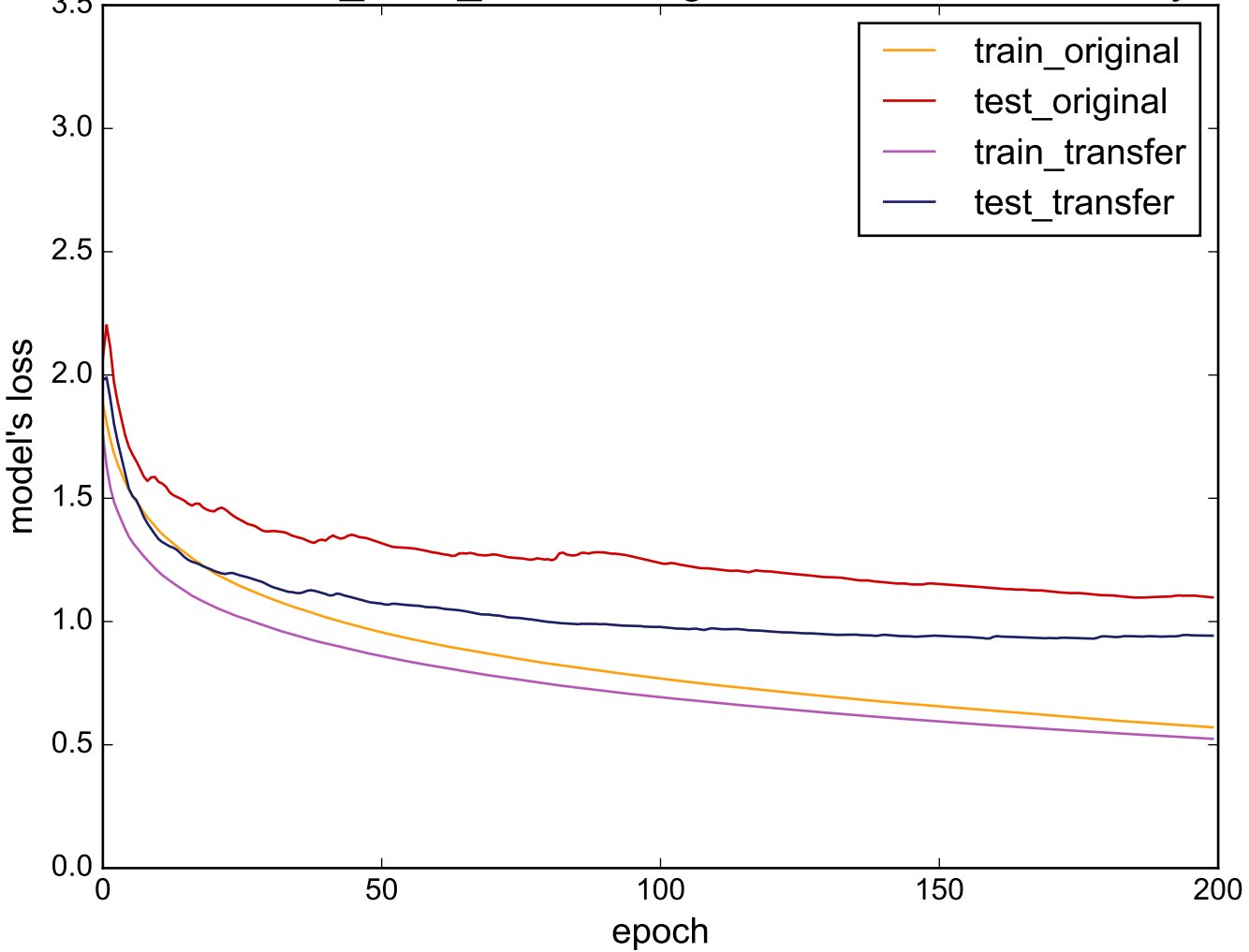
Source: CinC_ECG_torso - Target: UWaveGestureLibraryAll
