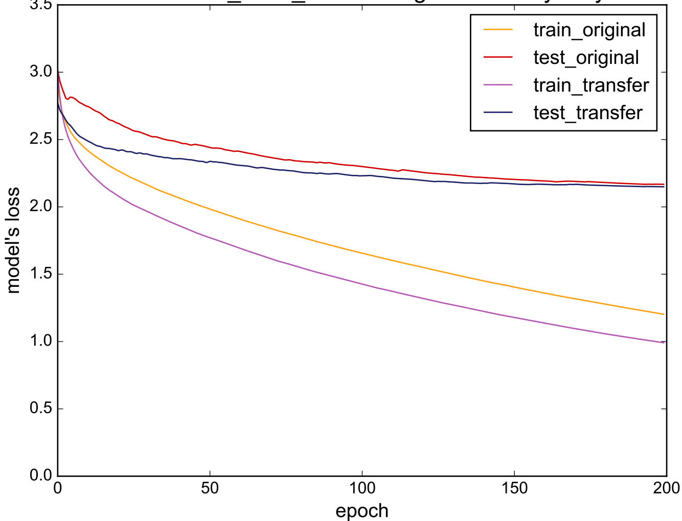
Source: CinC_ECG_torso - Target: WordsSynonyms
