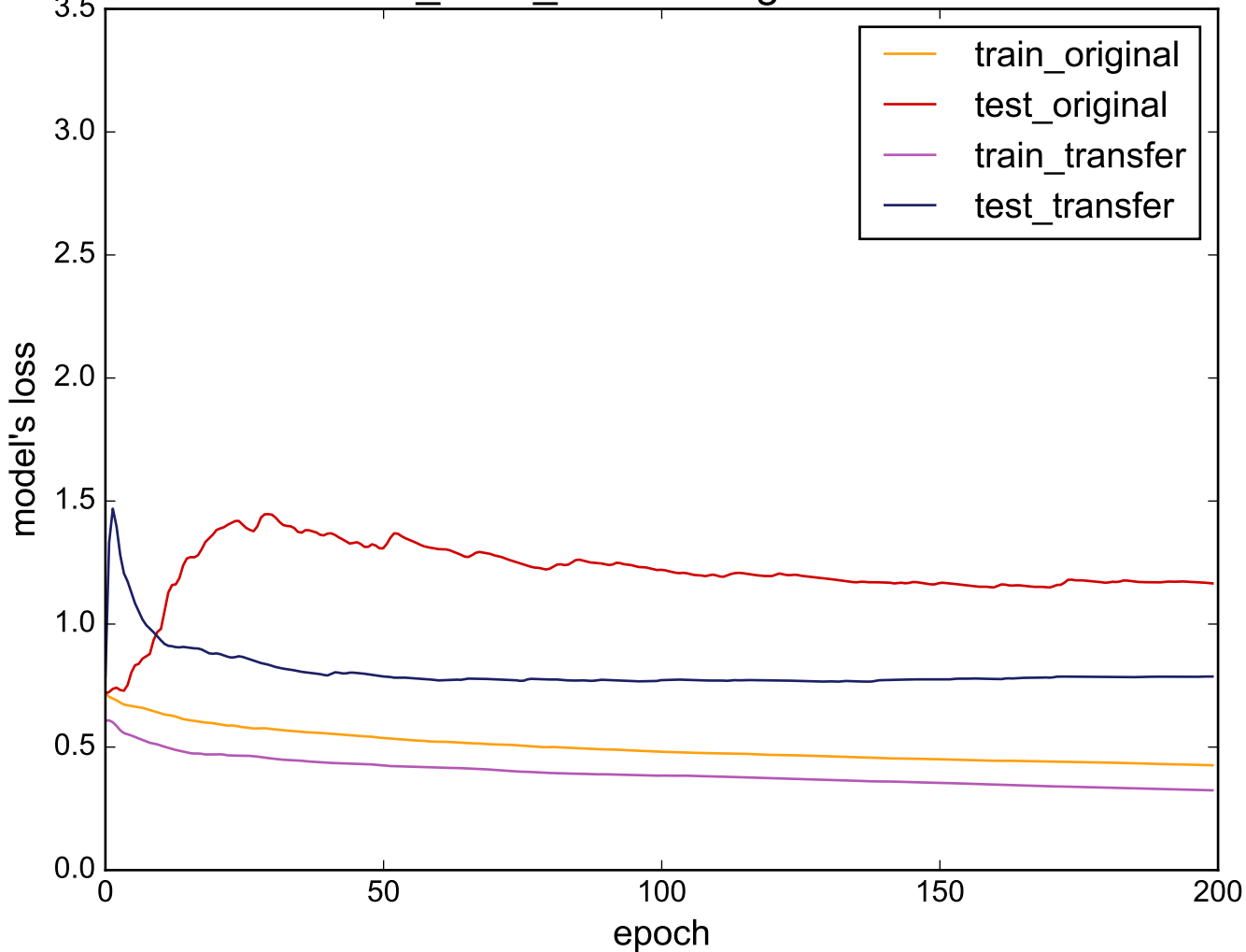
Source: CinC_ECG_torso - Target: WormsTwoClass
