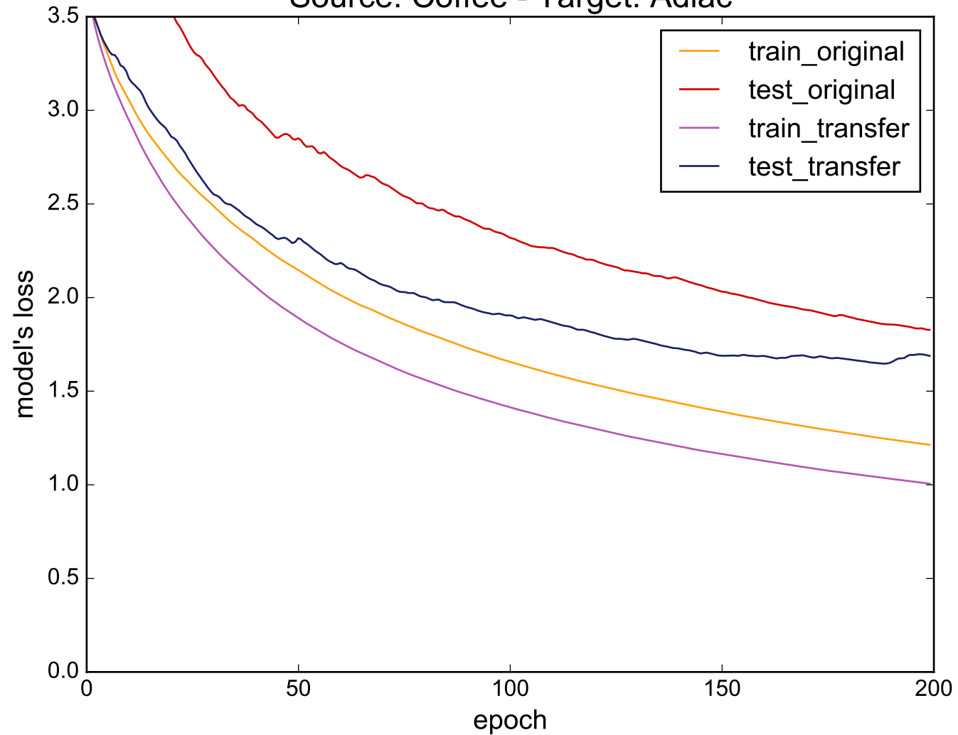
Source: Coffee - Target: Adiac
