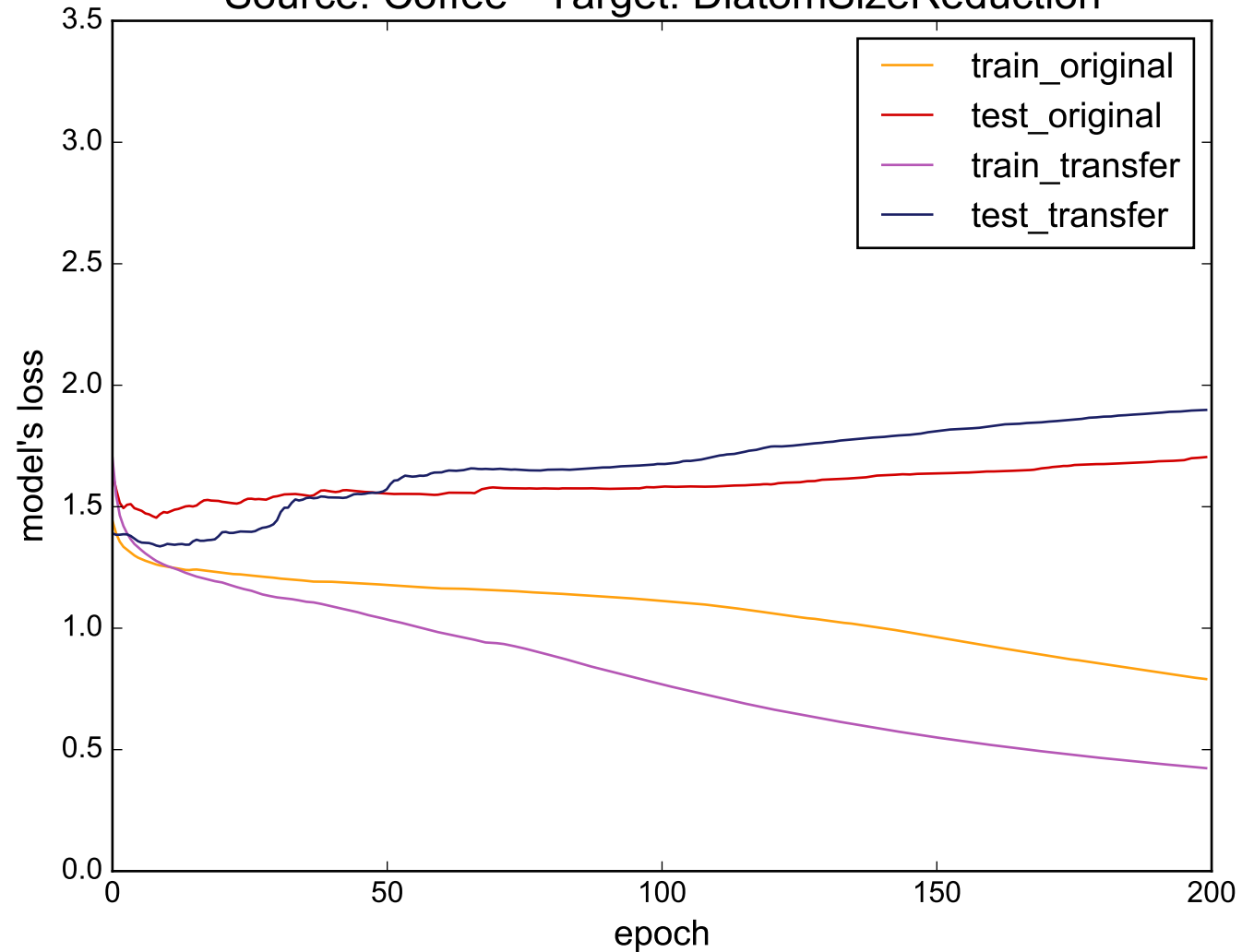
Source: Coffee - Target: DiatomSizeReduction
