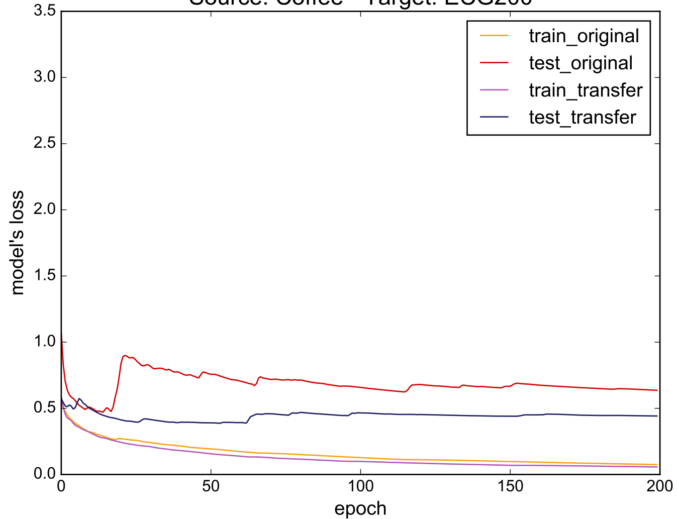
Source: Coffee - Target: ECG200
