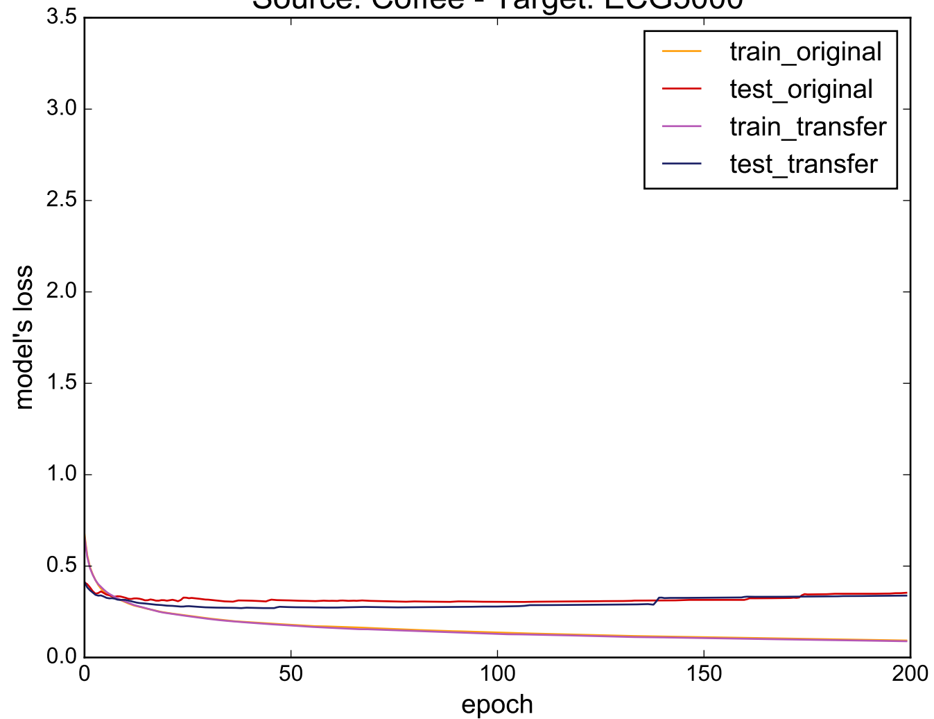
Source: Coffee - Target: ECG5000
