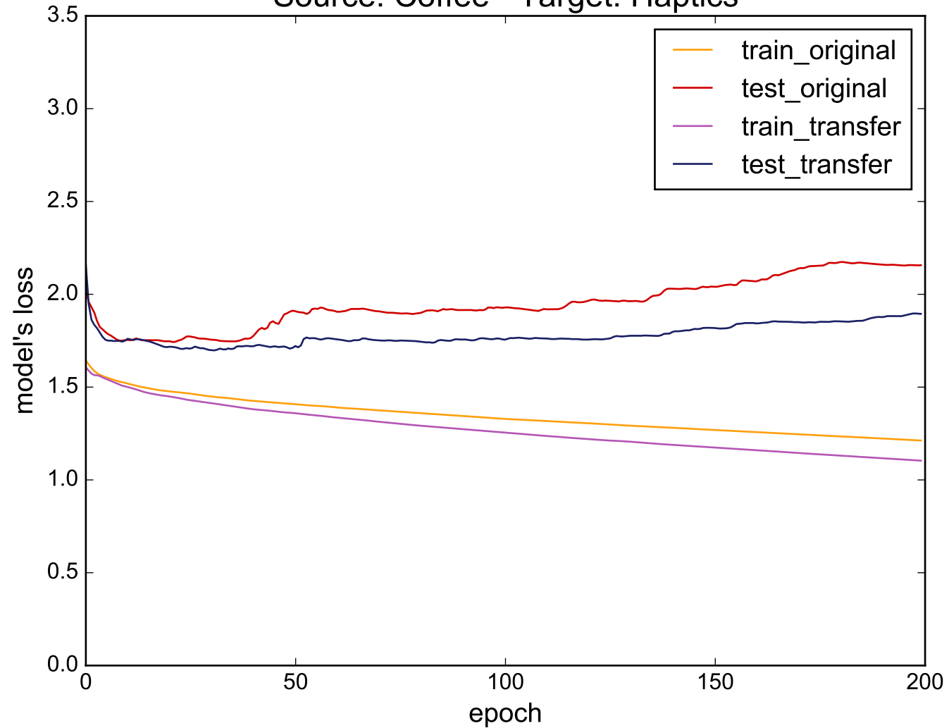
Source: Coffee - Target: Haptics
