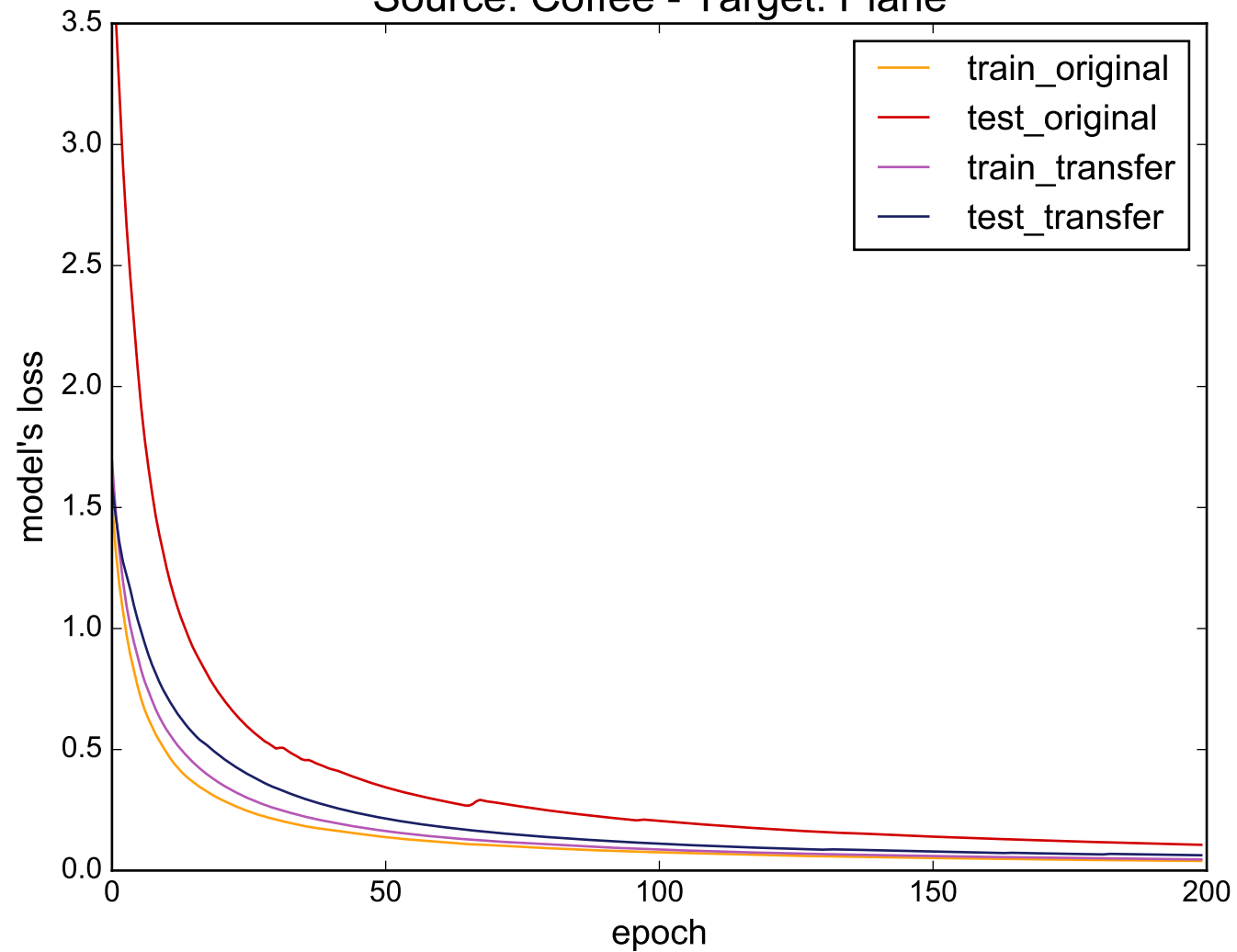
Source: Coffee - Target: Plane
