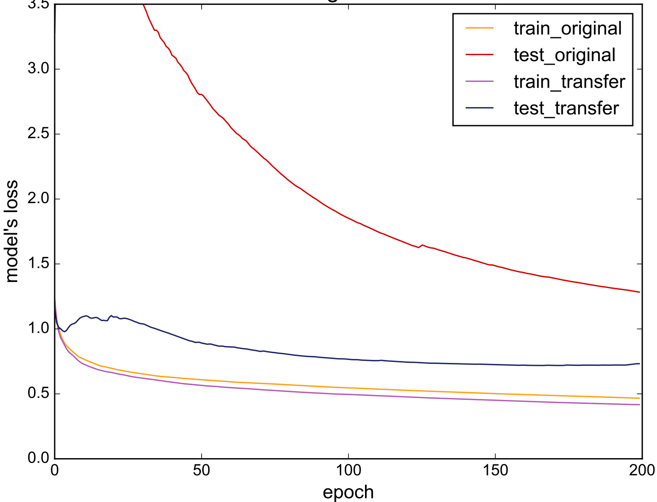
Source: Coffee - Target: ProximalPhalanxTW
