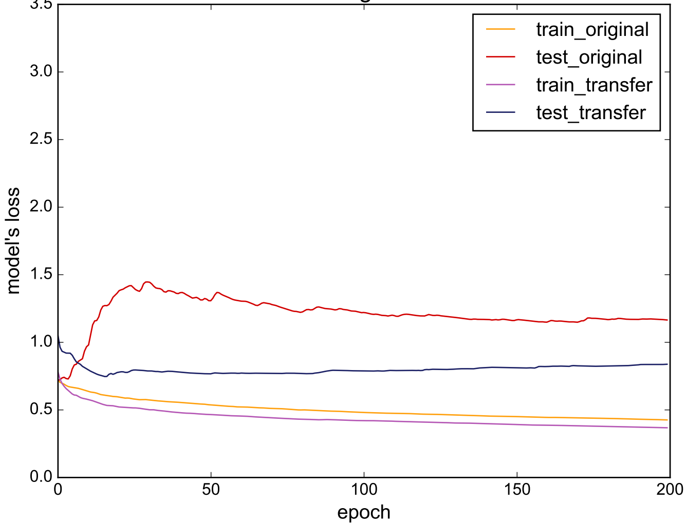
Source: Coffee - Target: WormsTwoClass
