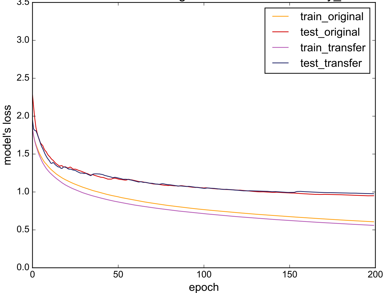
Source: Coffee - Target: uWaveGestureLibrary_X
