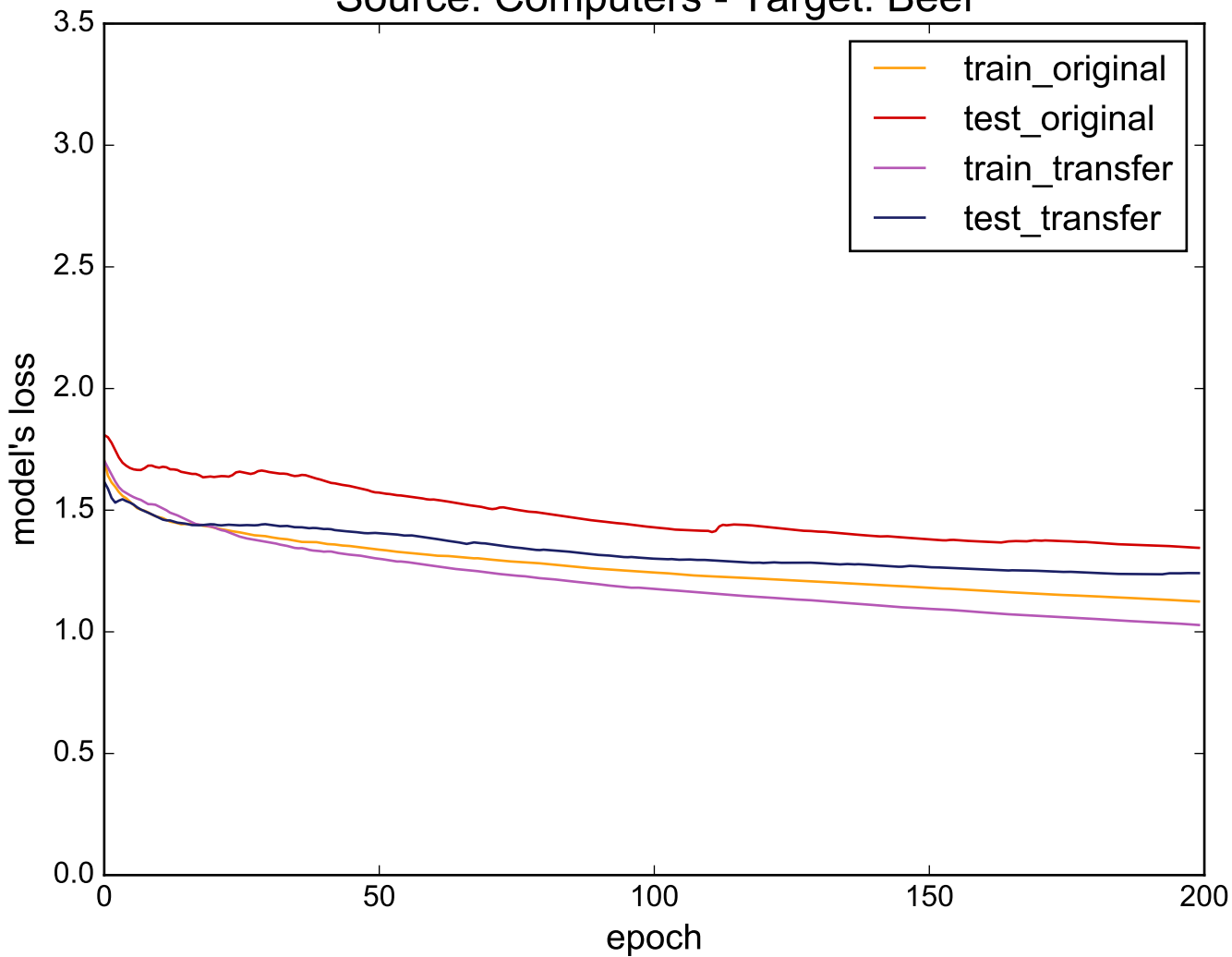
Source: Computers - Target: Beef
