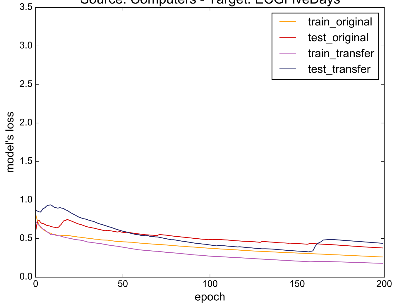
Source: Computers - Target: ECGFiveDays
