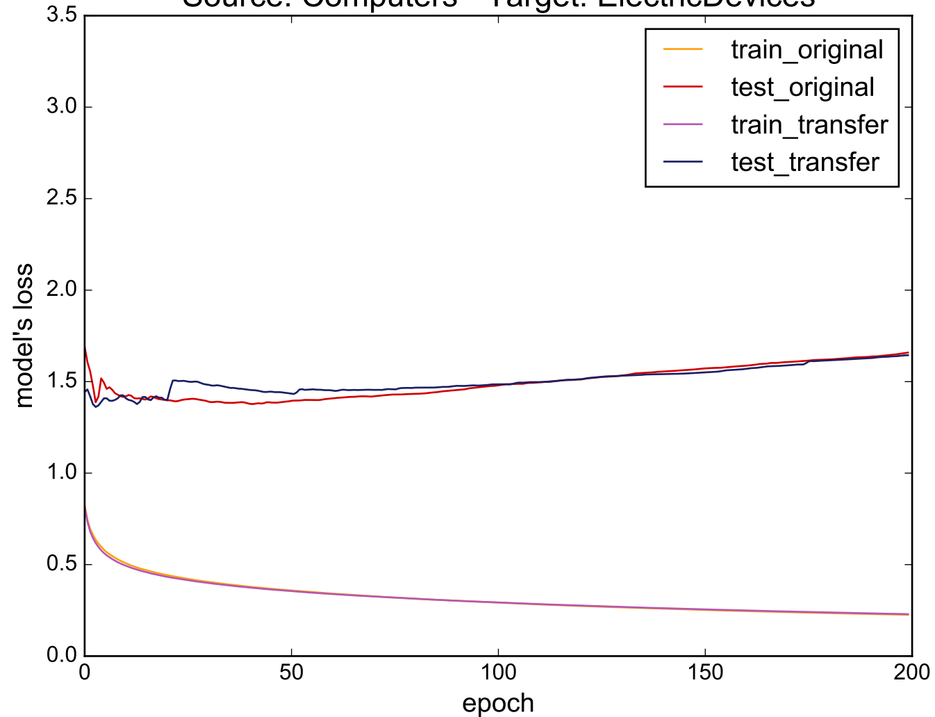
Source: Computers - Target: ElectricDevices
