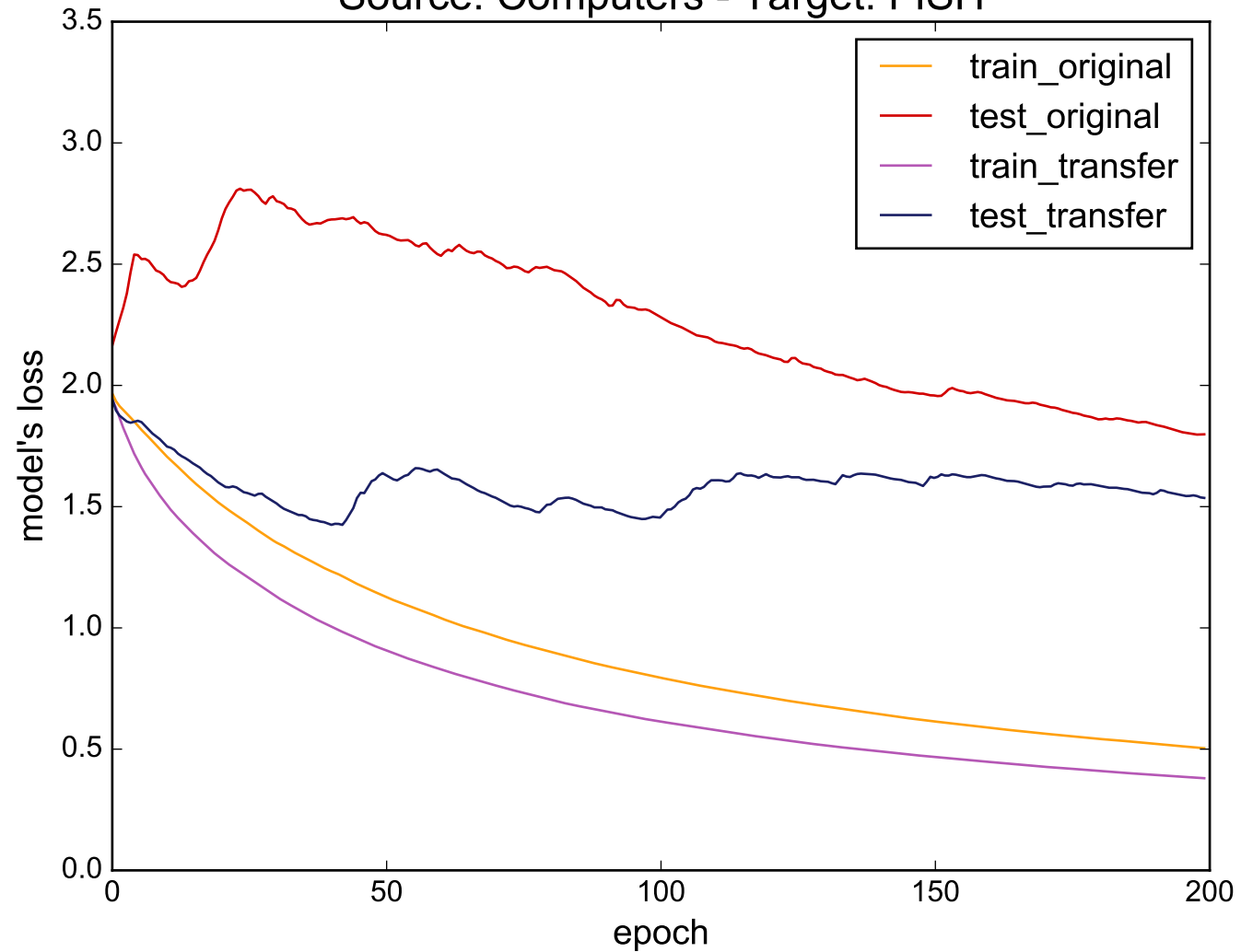
Source: Computers - Target: FISH
