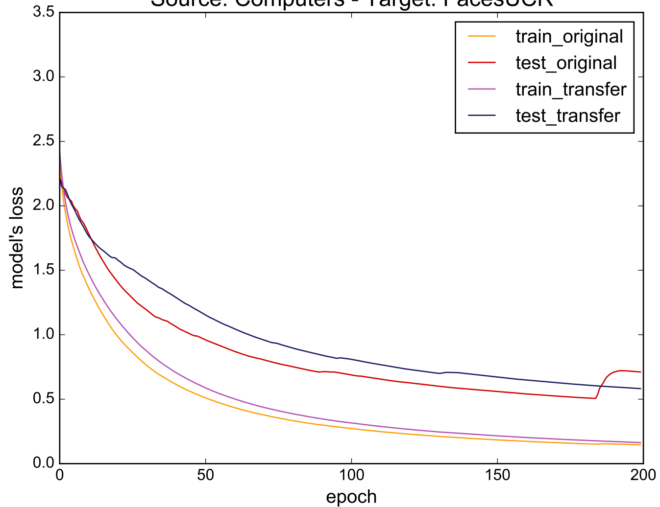
Source: Computers - Target: FacesUCR
