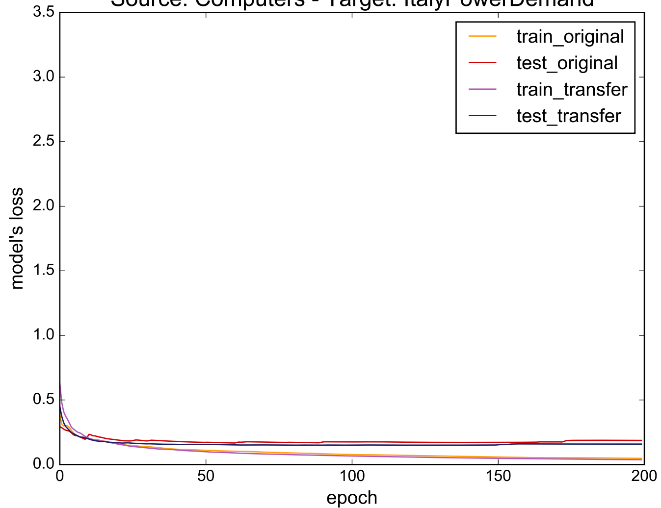
Source: Computers - Target: ItalyPowerDemand
