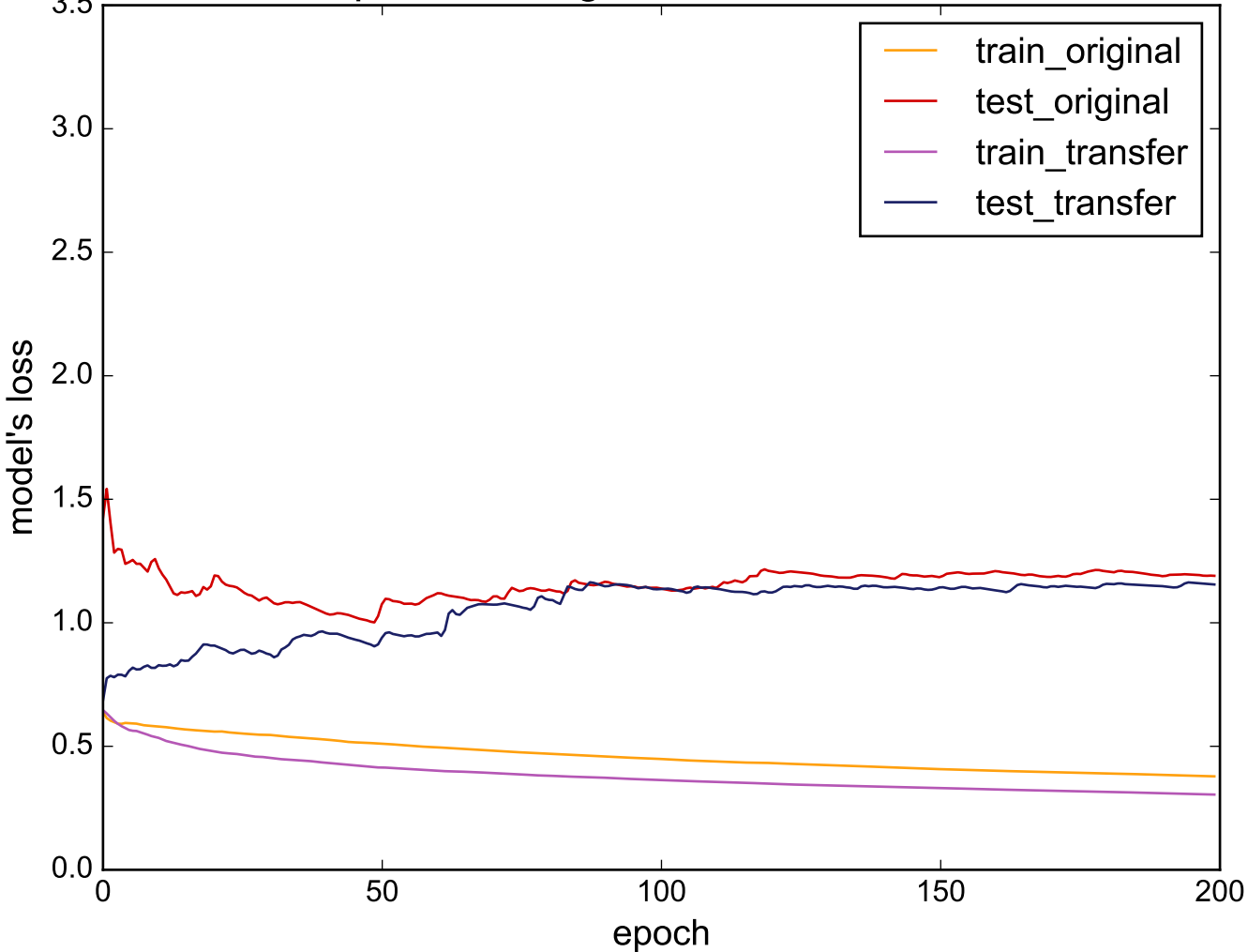
Source: Computers - Target: MiddlePhalanxOutlineCorrect
