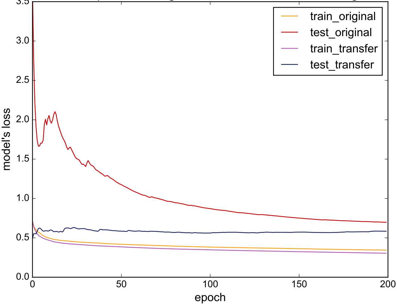
Source: Computers - Target: ProximalPhalanxOutlineAgeGroup
