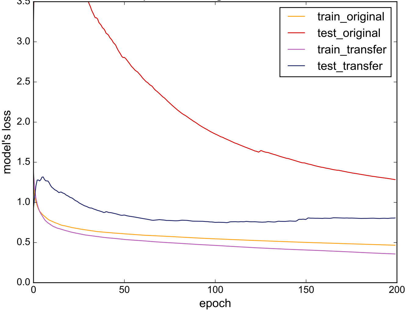
Source: Computers - Target: ProximalPhalanxTW
