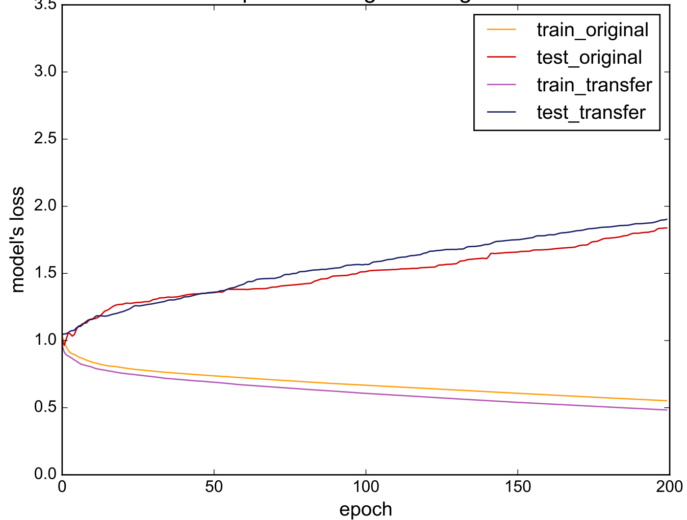
Source: Computers - Target: RefrigerationDevices
