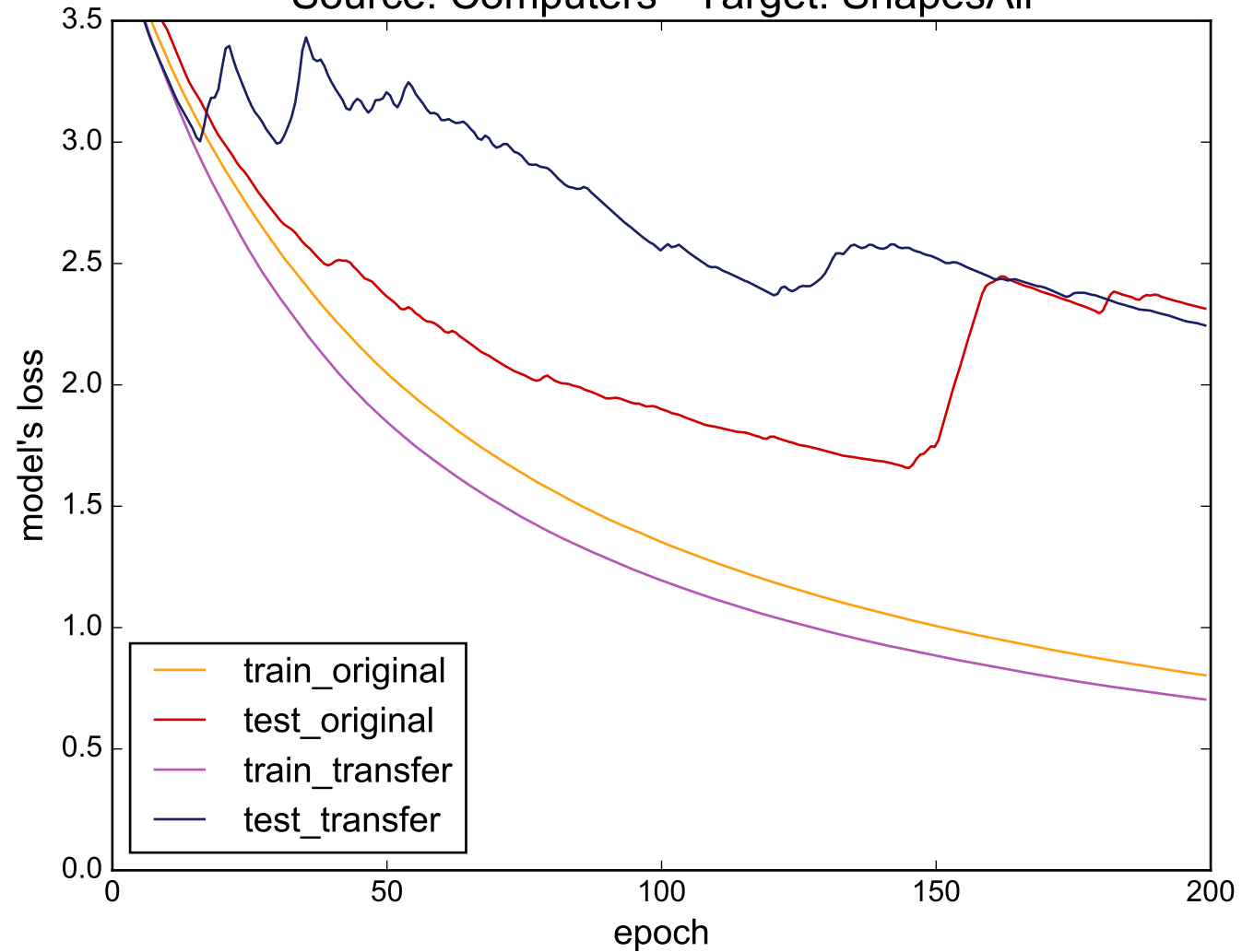
Source: Computers - Target: ShapesAll
