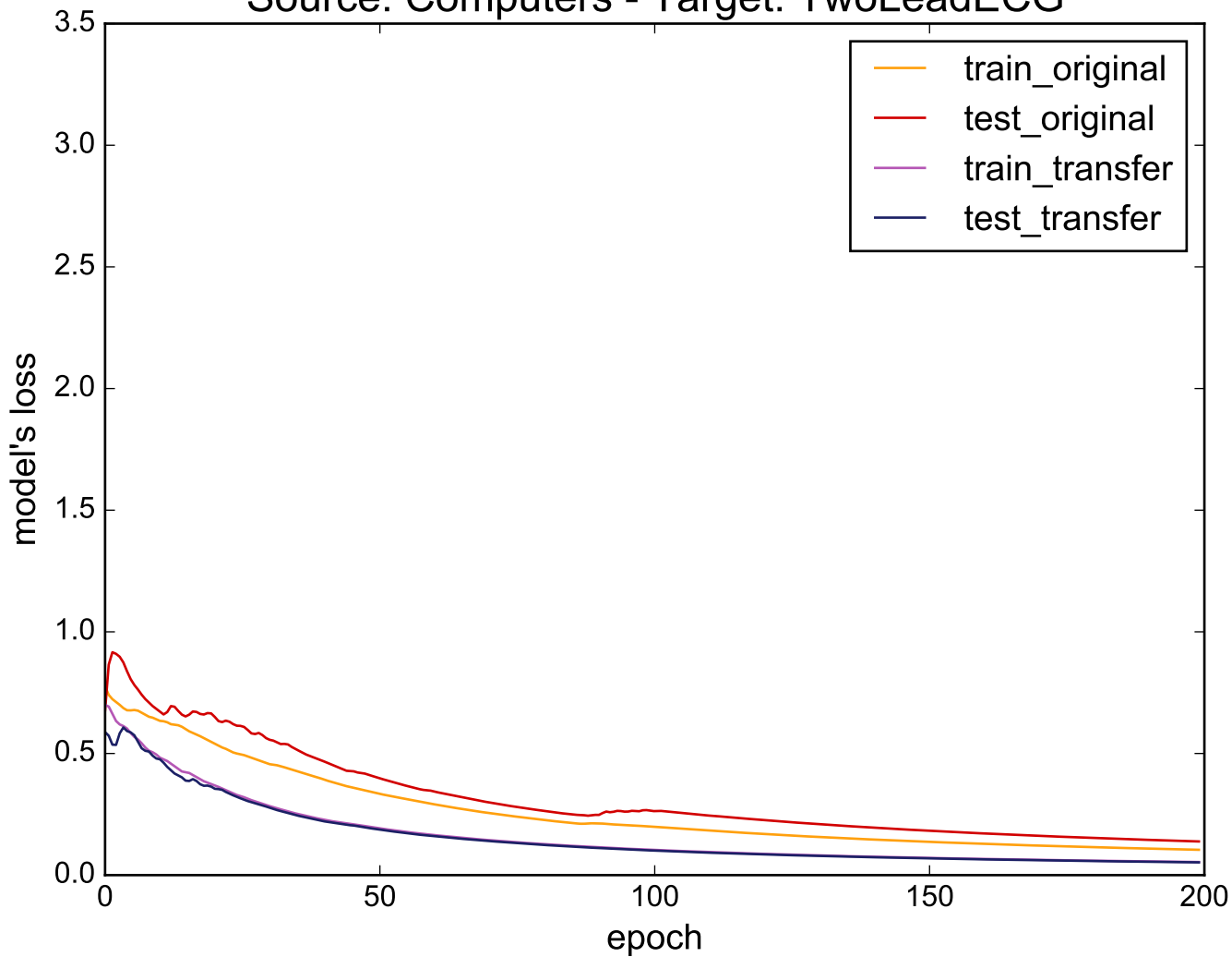
Source: Computers - Target: TwoLeadECG
