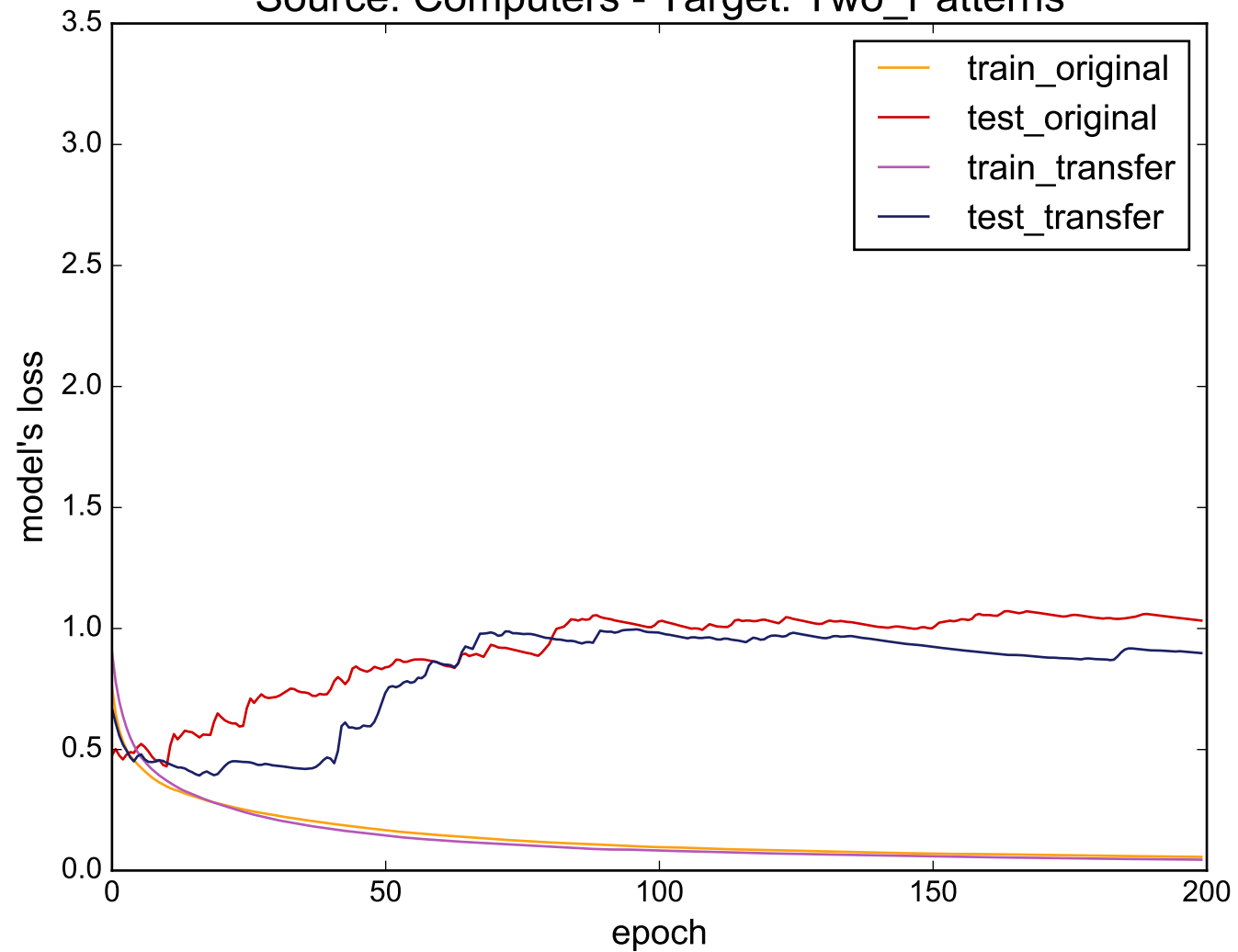
Source: Computers - Target: Two_Patterns
