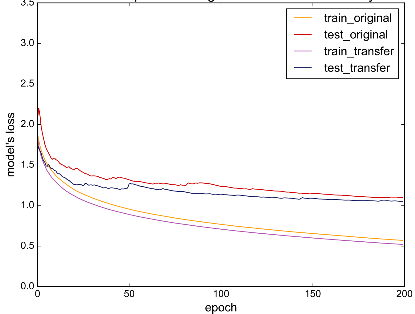
Source: Computers - Target: UWaveGestureLibraryAll
